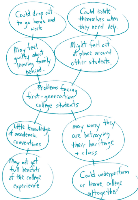
Figure 3.1 Clustering
