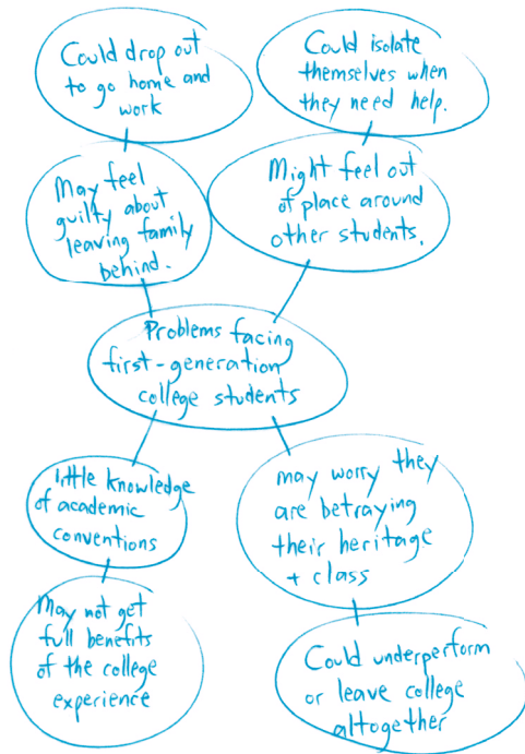
Figure 3.1 Clustering
